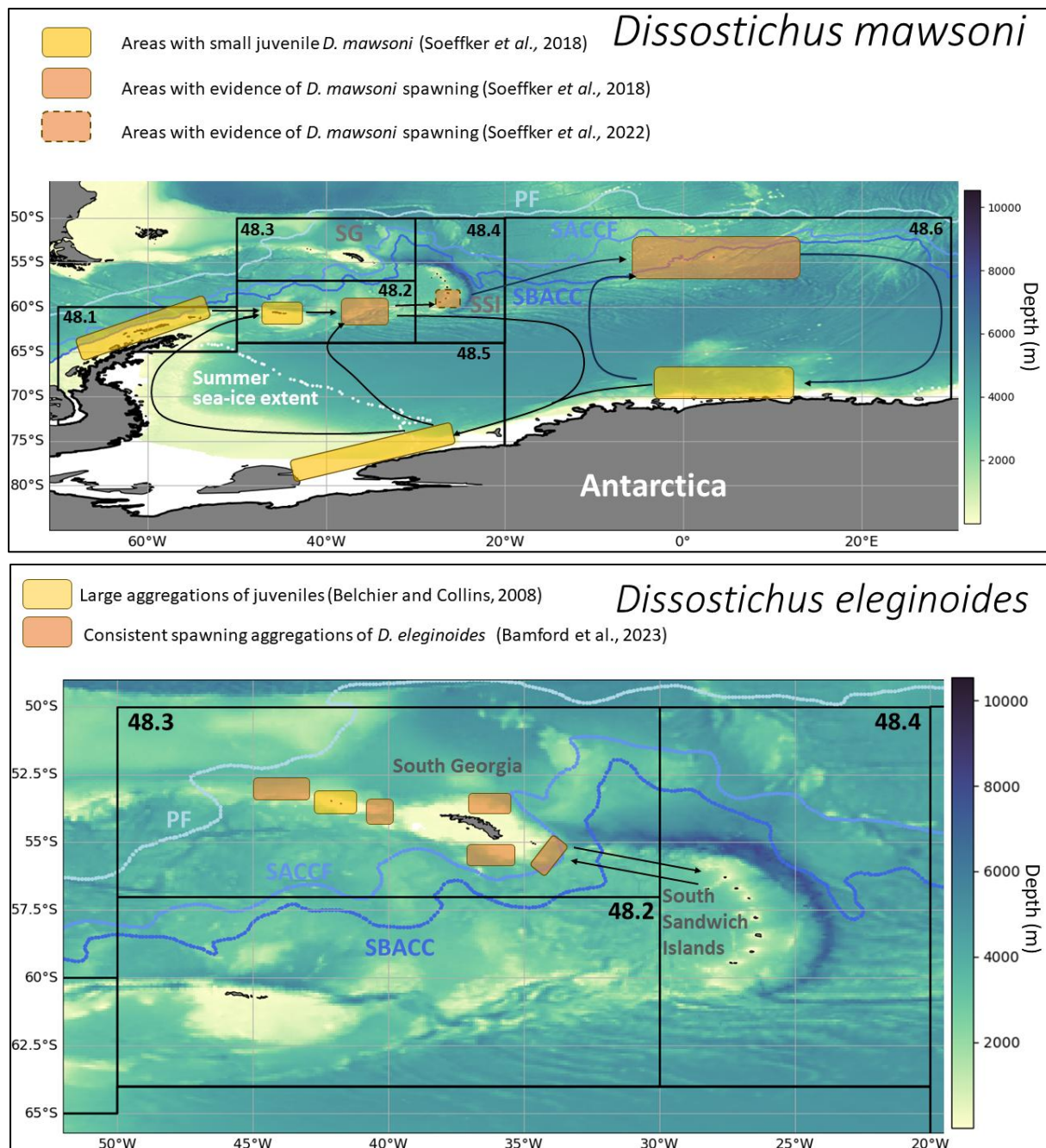
Figure 1: Stock hypotheses of Dissostichus mawsoni (top panel) and D. eleginoides (bottom panel) at SGSSI, based on existing literature. Hypothesised nursery (yellow shaded boxes) and spawning (orange shaded boxes) habitats are marked, along with migrations between habitats (black arrows). The distribution of the key habitats of both stocks are shown in relation to fishery management areas and oceanographic features. The extent of CCAMLR Area 48 and the Subareas are shown in black boxes. Summer sea-ice extent (white dotted line) is the median extent for February 1982-2010 (Fetterer et al., 2017). The mean positions of the Polar Front (PF), South Antarctic Circumpolar Current Front (SACCF), and Southern Boundary of Antarctic Circumpolar Current Front (SBACC) were calculated using satellite data from 1993-2012 (Park and Durand, 2019). Seafloor depth data is from E.U. Copernicus Marine Service Information; https://doi.org/10.48670/moi-00021
